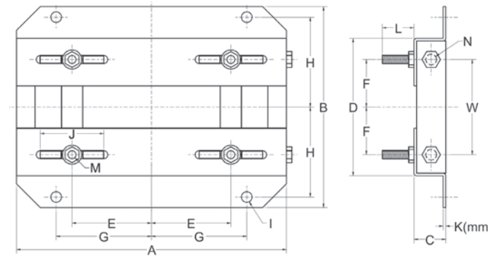
Dual adjusting screws on frames 182T-505T
